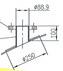
DETAIL OF N3, N6 SCALE 1:15
